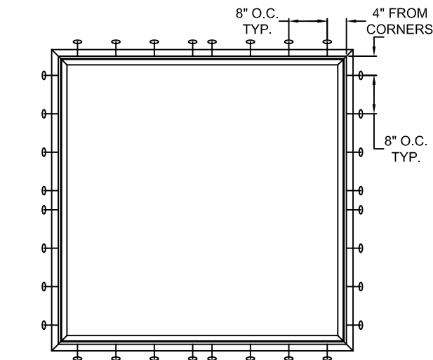
TYPICAL ELEVATION WITH FASTENER SPACING
